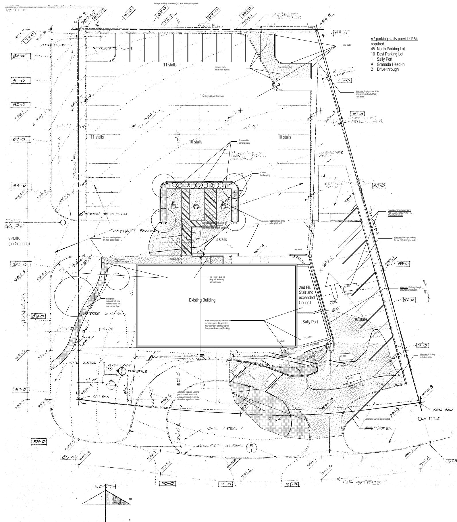
1 Site Plan 1/8" = 1'-0"
